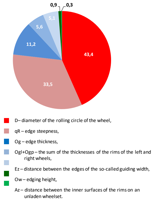
Fig. 6. Percentage of exceeding a given ZK parameter to all exceedances of geometrical parameters found in time P2
