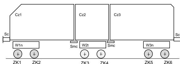
Fig. 1. Scheme of one of the two EN97 three-sections of the vehicle: Cz1 – drive unit with a control cabin, Cz2 – central rolling member, Cz3 – drive unit without a control cabin, W1n, W3n – bogies, W2t – central rolling bogie, ZK1–ZK6 – wheel sets, Sc – front coupler, Smc – inter-unit coupler
