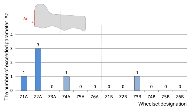
Fig. 13. The number of violations of the parameter of the distance between the inner surfaces of the rims in the unloaded wheelset Az during inspections P2
