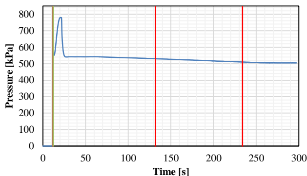
Fig. 10. Change of pressure in the brake pipe as a function of time during high pressure release
