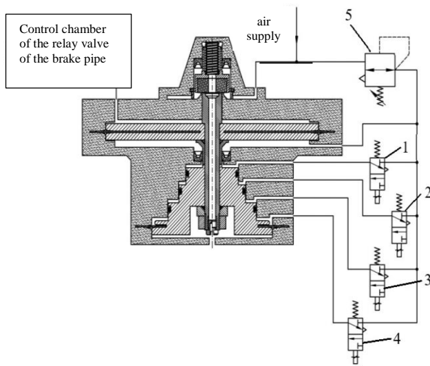
Fig. 1. Electro-pneumatic brake pipe pressure control system: 1, 2, 3, 4 – electro-pneumatic valves, 5 – reducing valve [6]
