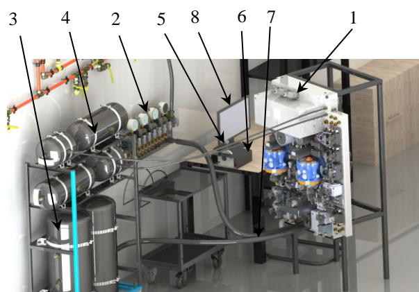
Fig. 3. Test stand of the pressure control system in the brake pipe
