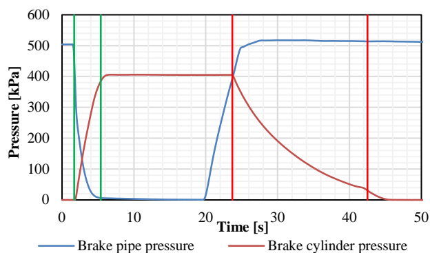
Fig. 8. Changing the pressure in the brake pipe as a function of time in the "Passenger" setting
