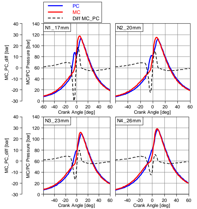
Fig. 6. Indicator diagrams for subsequent prechamber neck diameter
